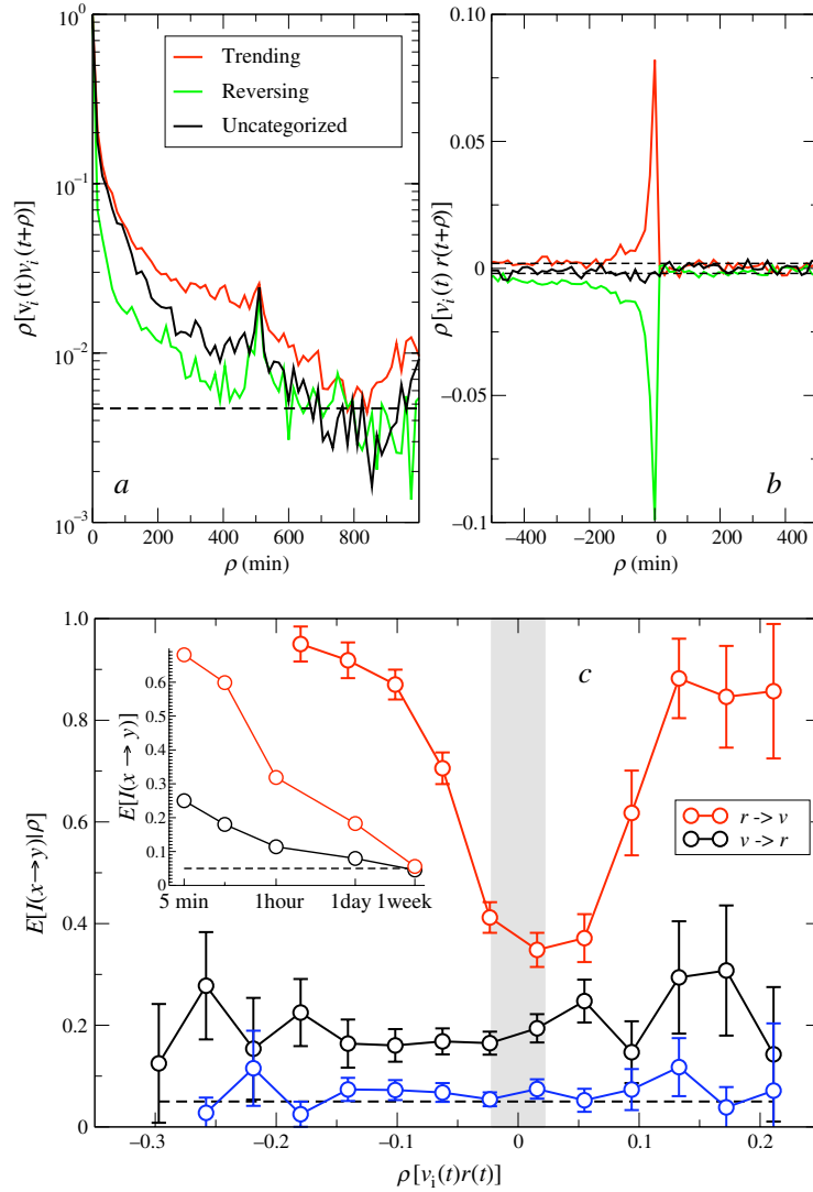
Figure 4. Panels (a) and (b) show the averaged autocorrelation of v_i(t) and averaged lagged cross-correlation \rho[v_i(t), r(t+\tau)] (respectively) for the different firm groups. The dashed lines bound the 2\sigma significance interval. In panel (c), we show the conditional expected value of the indicator I(X \rightarrow Y) of the rejection of the null hypothesis of non-Granger causality between X and Y with 95% confidence as a function of the simultaneous cross correlation \rho[v_i(t), r(t)] . Red symbols refer to the test that r(t) is Granger-causing v_i(t) whereas black symbols refer to the test that v_i(t) is Granger-causing r(t) . Granger-causality is tested on the time series of v_i(t) and r(t) obtained at each \Delta t = 15 min and over p = 10 lags, corresponding to 150 min. The blue line is a result of the Granger test on shuffled data. The shaded area corresponds to values of \rho within the \pm 2\sigma significance level. The inset shows the average value of the indicator for other time horizons \Delta t with p = 10 and the same color code as before. The dashed line is the value 0.05 expected for a test of a null hypothesis performed by using a 95% confidence level.
