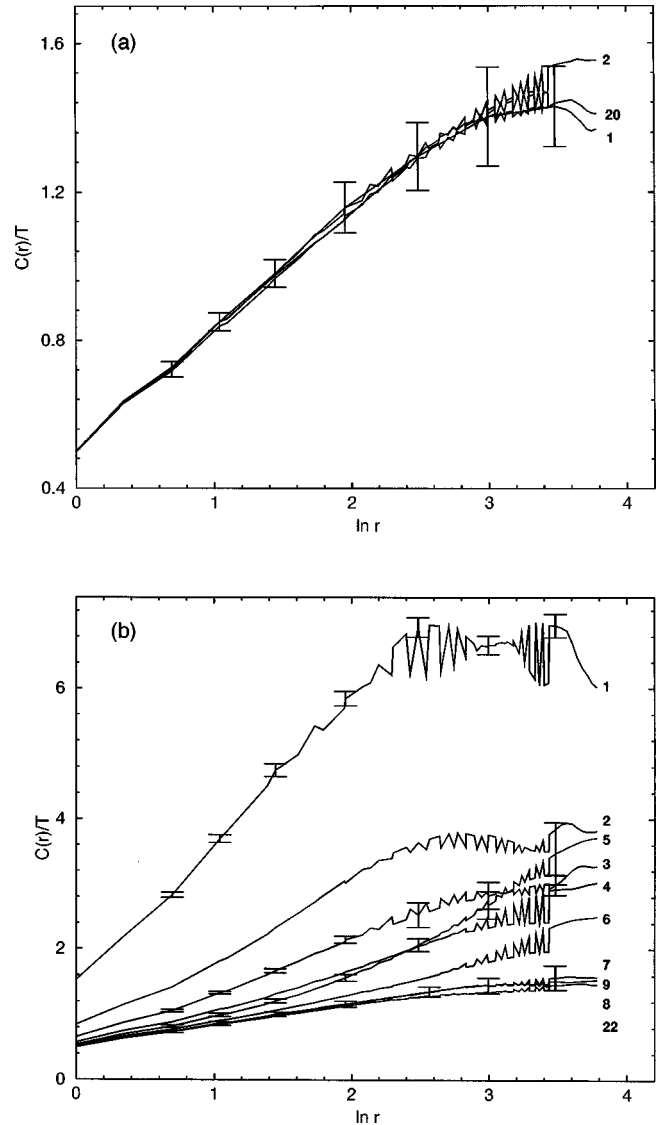
FIG. 7. Comparison of the height difference correlation functions for the RSGM with V_0=0.2 (upper panel), and V_0=5 (lower panel). Temperatures as indicated in the plots.
